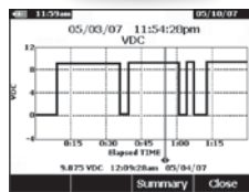
Switching signal from a dc voltage relay output
