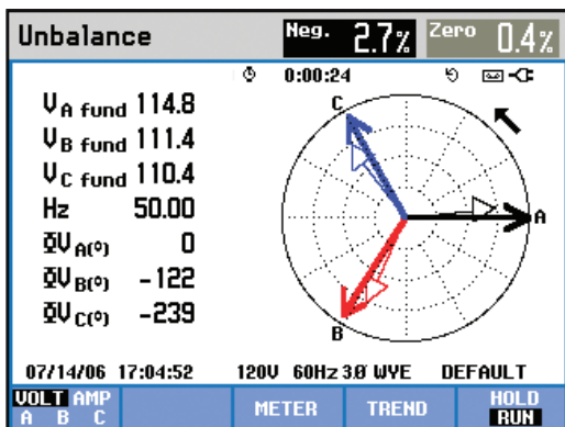
Phasor diagram shows voltage and current unbalance, and helps verify connections.
