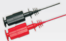
BP-266 (HV IC Clip, 7KV RMS, 3A 208L x 44W x 38H mm)
