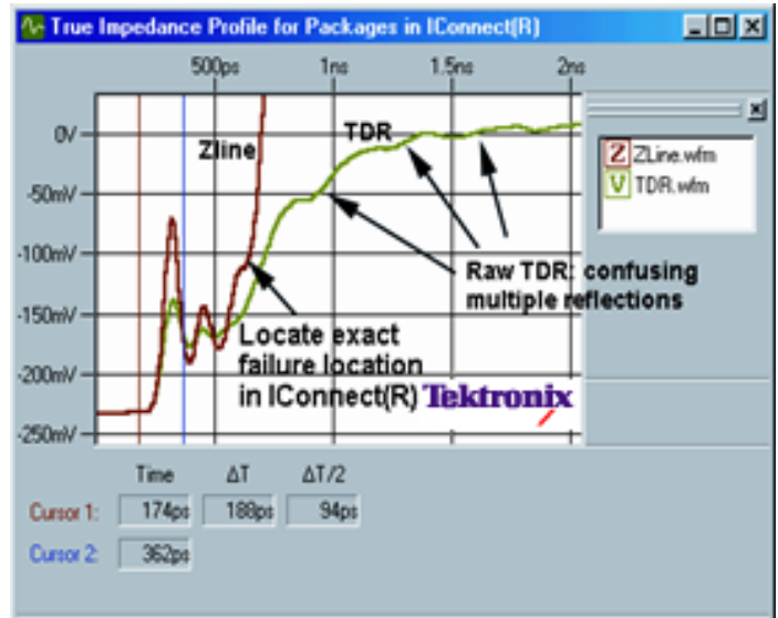
Quickly identify the exact location of faults with the 80E10's sub-millimeter resolution and IConnect True Impedance Profile.
