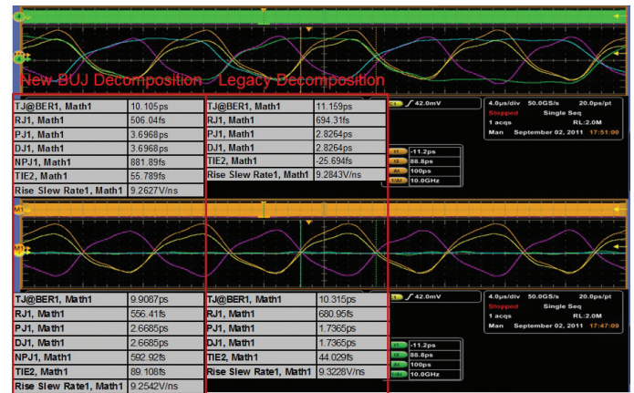
Figure 4.2.6. Improved TJ and greater margin using Bounded, Uncorrelated Jitter separation methodologies.
