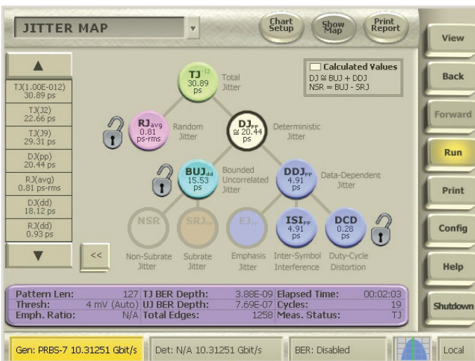
Figure 2.4d. BERT with Jitter Values on
