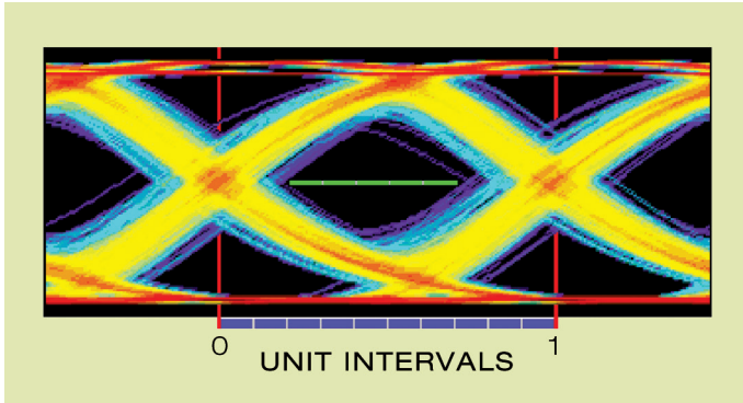
Figure 5.2a. Eye Width is used to Determine Performance.
