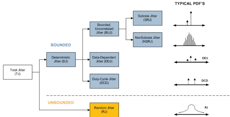
Figure 4.2. Jitter is Composed of Random and Deterministic Parts.
